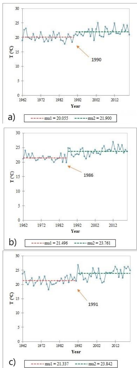
Figure 4: Pettit's test results for mean monthly air temperatures in June (a), July (b) and August (c) in Belgrade (1961-2020)
